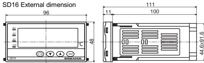
SD16 External dimension
